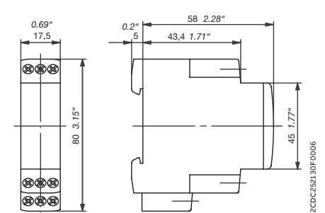
CT-C devices with 2 c/o contacts
