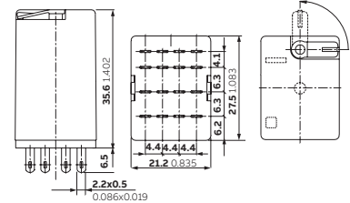
CR-M relay with 4 c/o contacts
