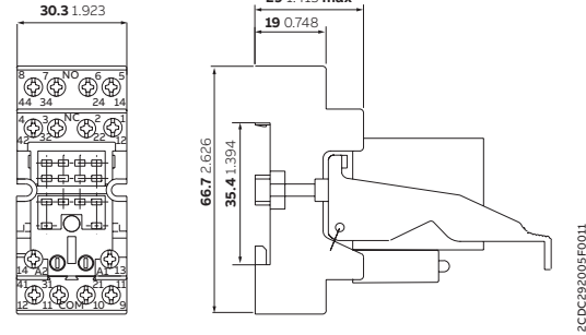
CR-MxSF - screw connection
