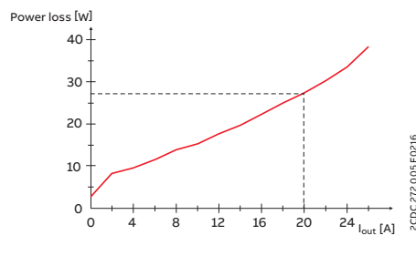
Typical power loss over output current
